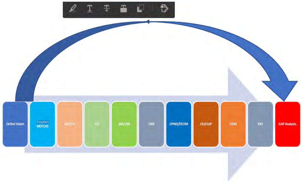
Figure 1: Project's phases.
