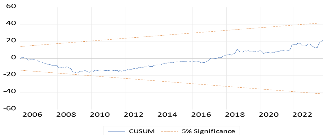
Figure 2. CUSUM test results of ARDL (1,1,0,0,1) model
