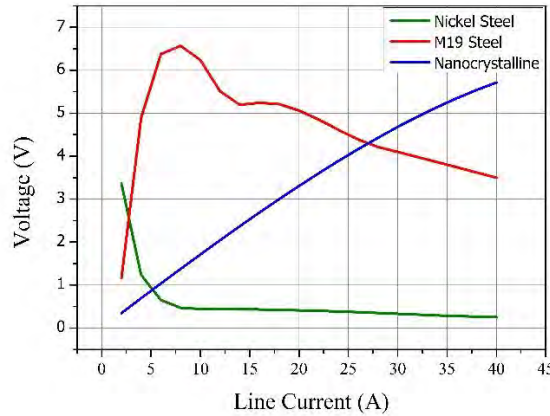
Figure 6. Induced voltage.
