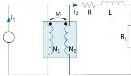
Figure 3. Equivalent circuit of harvester.
