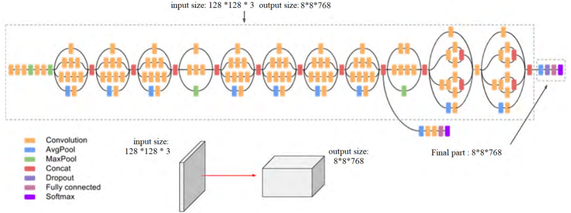
Figure 2. Explain the IncptionV3 design [14].
