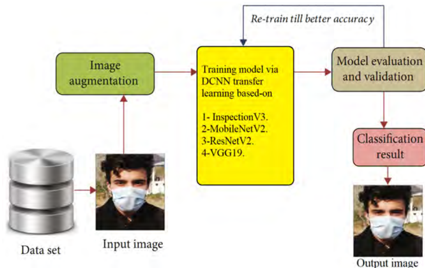
Figure 1. Illustrate the diagram of this study.
