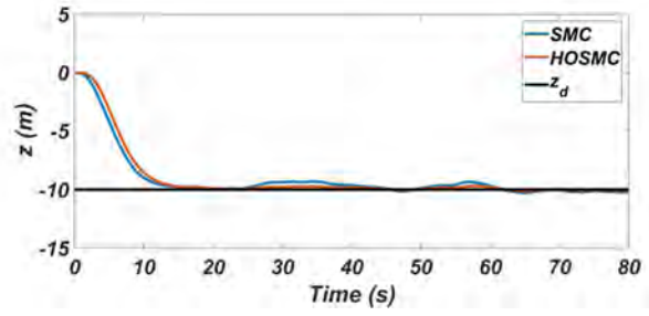
Figure 14. Depth control of robot with HOSMC in disturbed environment
