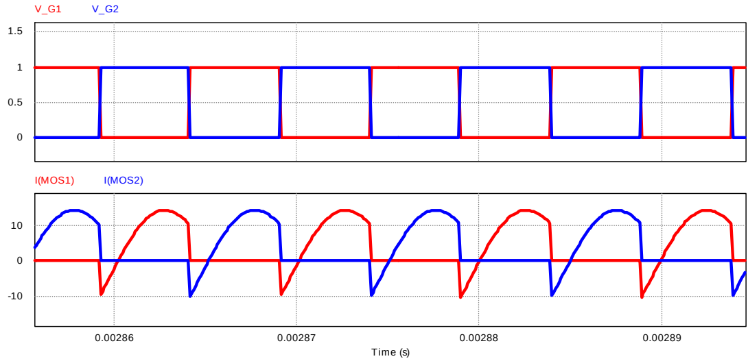
Figure 7. Simulation results for f_s = 1.1f_r in a class D voltage source series resonant inverter
